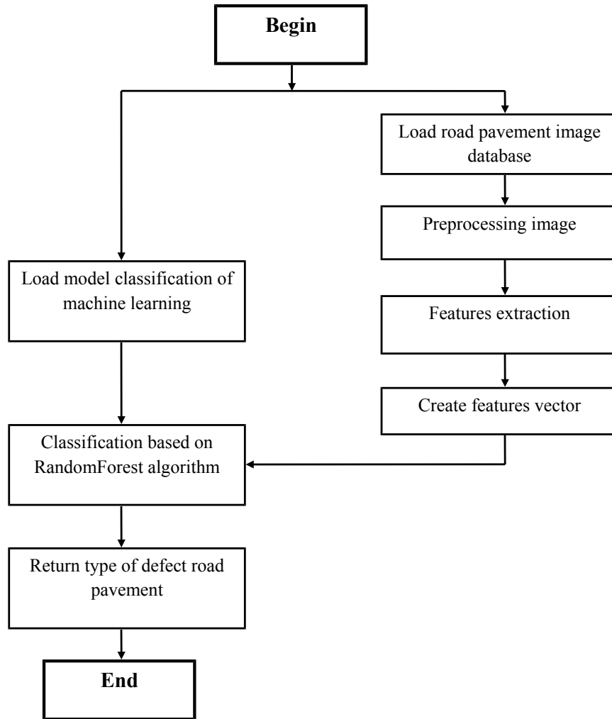
Fig. 5. Defect of pavement classification flow-chart.
